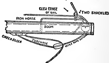
GEAR FOR HAULING OUT LOOSE-FOOTED MAINSAIL.
